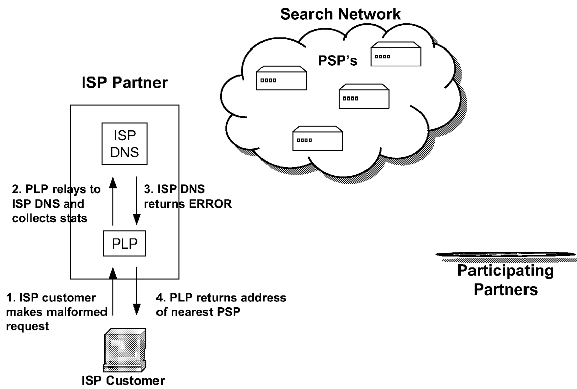
FIG. 2 - Customer Makes Malformed Request
