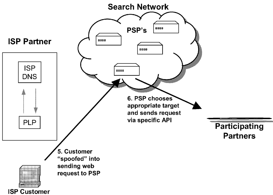
FIG. 3 - Customer Sends Web Request To PSP
