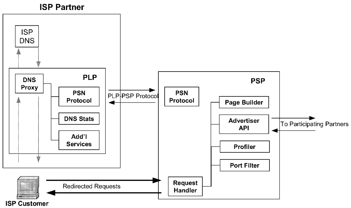
FIG. 7 – Overall Architecture
