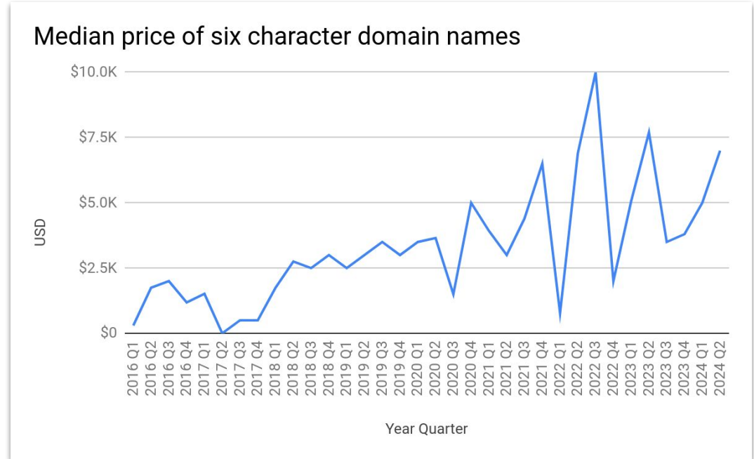
Figure 12: Median price of six character domain names (Escrow.com)
