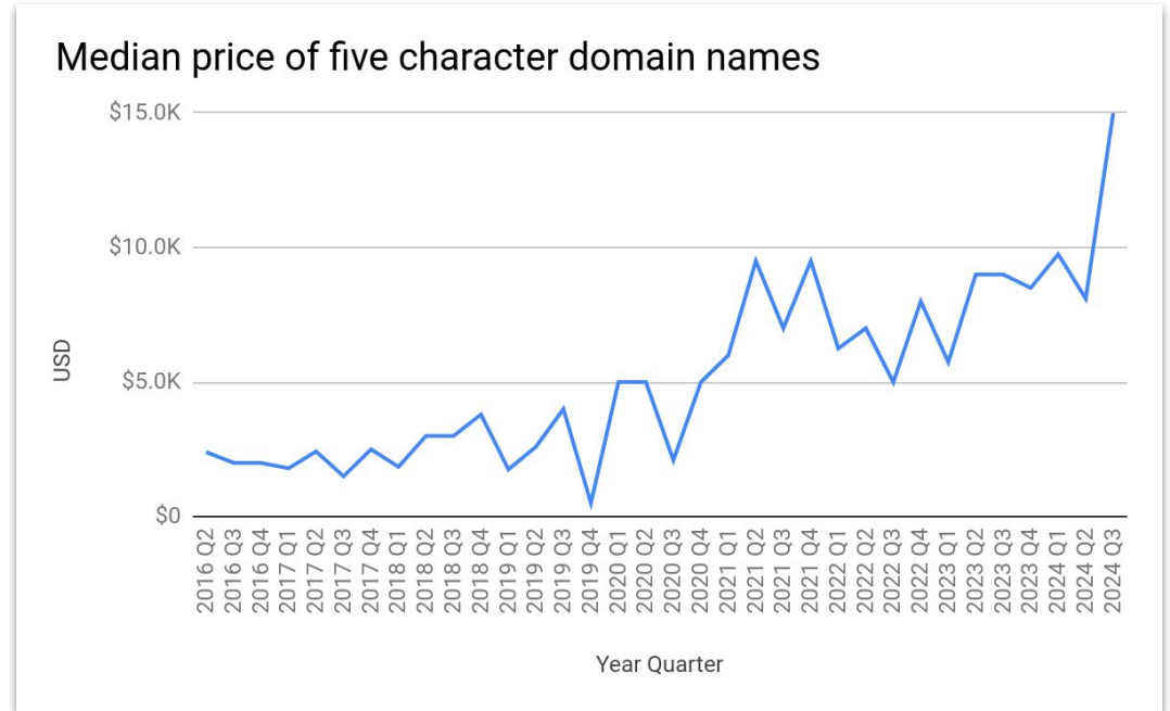
Figure 11: Median price of five character domain names (Escrow.com)
